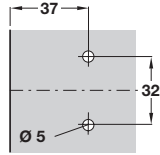
With pre-mounted Euro screws
