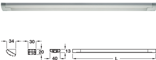
Loox 24V LED 3019 surface mounted strip light, 512 / 812 mm
