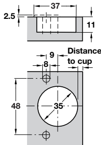
Dowel fixing
