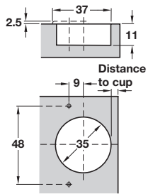
Screw fixing
