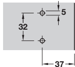
With pre-mounted Euro screws
