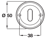
Standard keyway escutcheon
