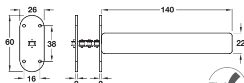
Radius plate
