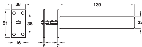
Radius plate
