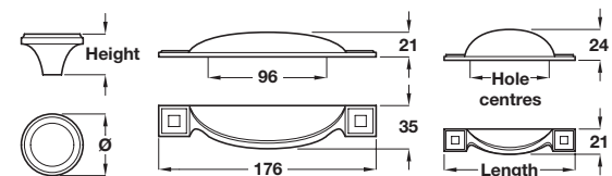
Knob, round
