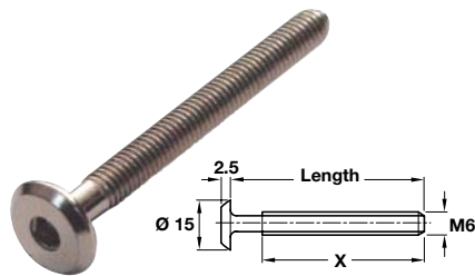
A M6 connecting bolt, flat ended
