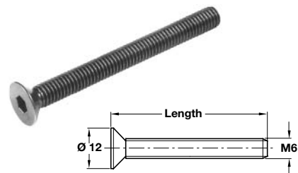
B M6 connecting bolt, countersunk
