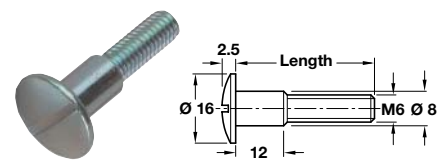
H M6 shoulder screw
