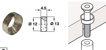
C Countersunk collar
