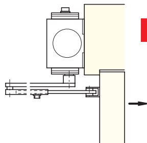
Fig 61 Transom application Closer is fixed to the push side of the door (overhead installation)
