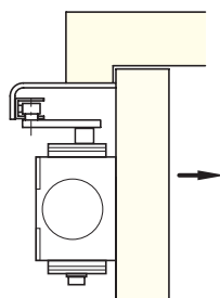
Fig 66 Parallel arm application Closer is fixed to the push side of the door using fixing bracket
