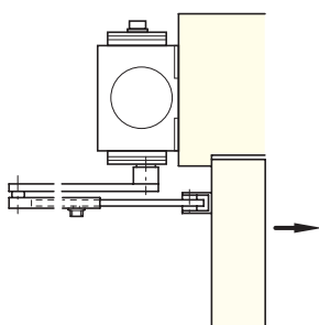
Fig 61 Transom application Closer is fixed to the push side of the door (overhead installation)
